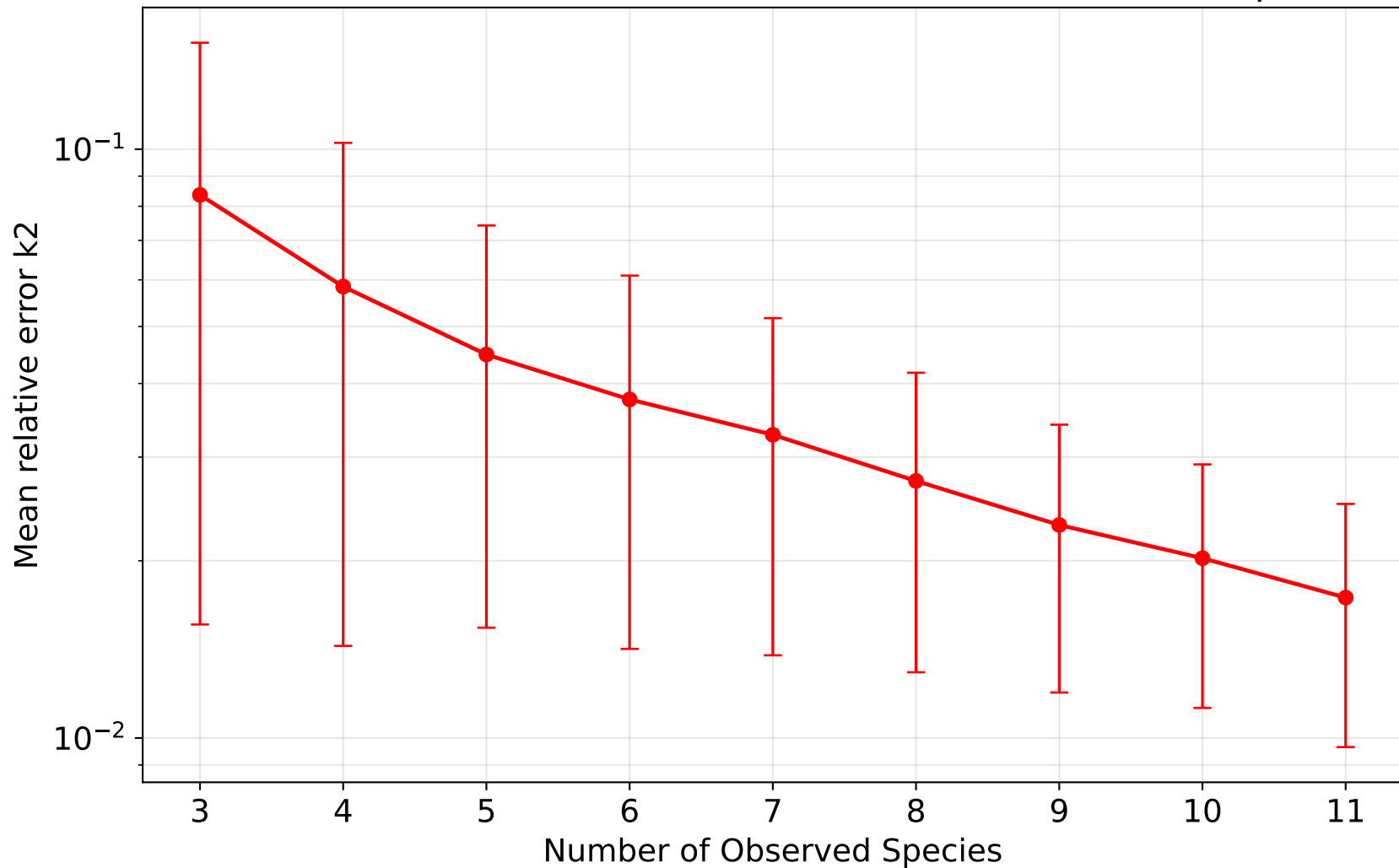
50, 50 — Mean relative error k2 vs number of observed species
